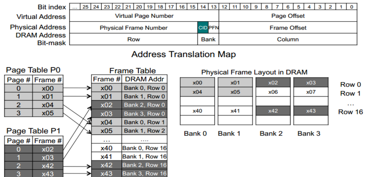
Figure 2-7 Bank Partition Frame Allocation
