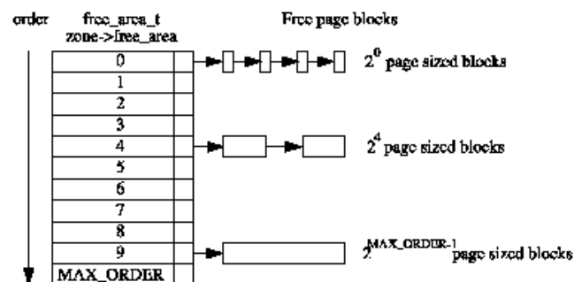
Figure 3-2 Zone to Buddy Page order Mapping
