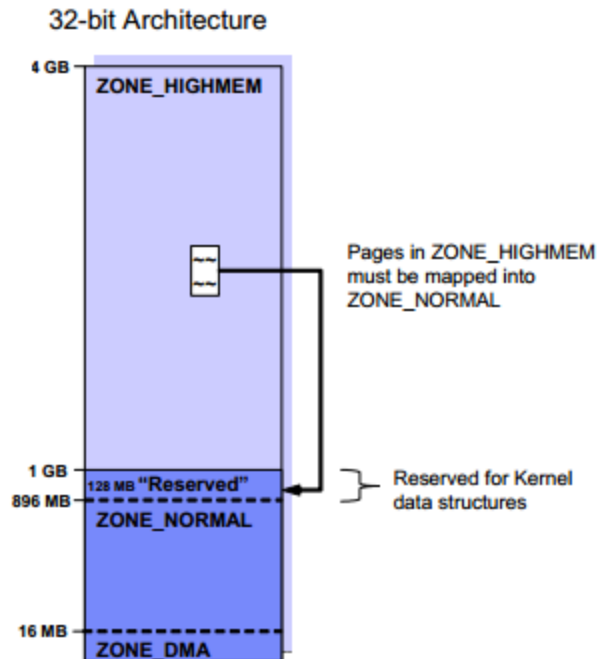
Figure 2-3 32 Bit Memory Zone
