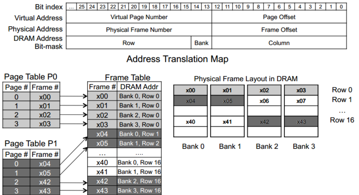
Figure 2-6 Virtual to physical DRAM
